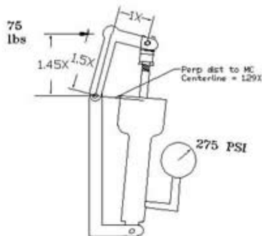
FIG 2 MECH ADV = 1.45/1.29 = 1.12 TO 1
