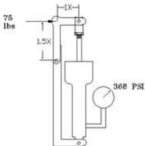
FIG 1 MECH ADV = 1.5/1 = 1.5 to 1
