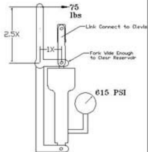
FIG 2 Minimum Geometry
