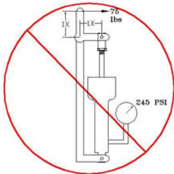
FIG 1 Poor Geometry
